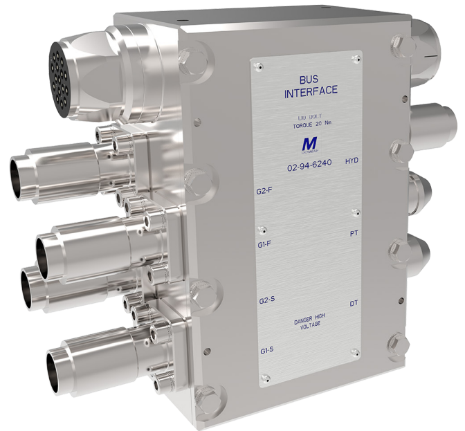
Gun Firing & Sensing Module (GFSM)
